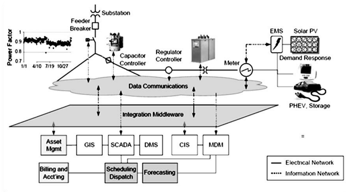
Fig. 2. Systems required supporting the SMART GRID [4].
