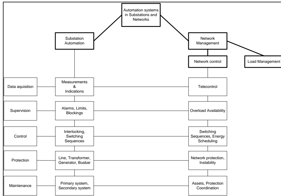
Fig. 1. Automation in substations and networks: functions and subsystems [8].
