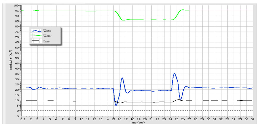
Fig. 3. Generator voltage response to a step signal
