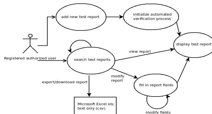
Fig. 1. Use-case view on the testing module for a user with full rights.
