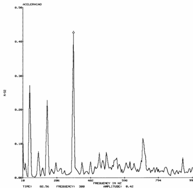
Fig. 1 Frequency spectrum (quick finishing moment)
