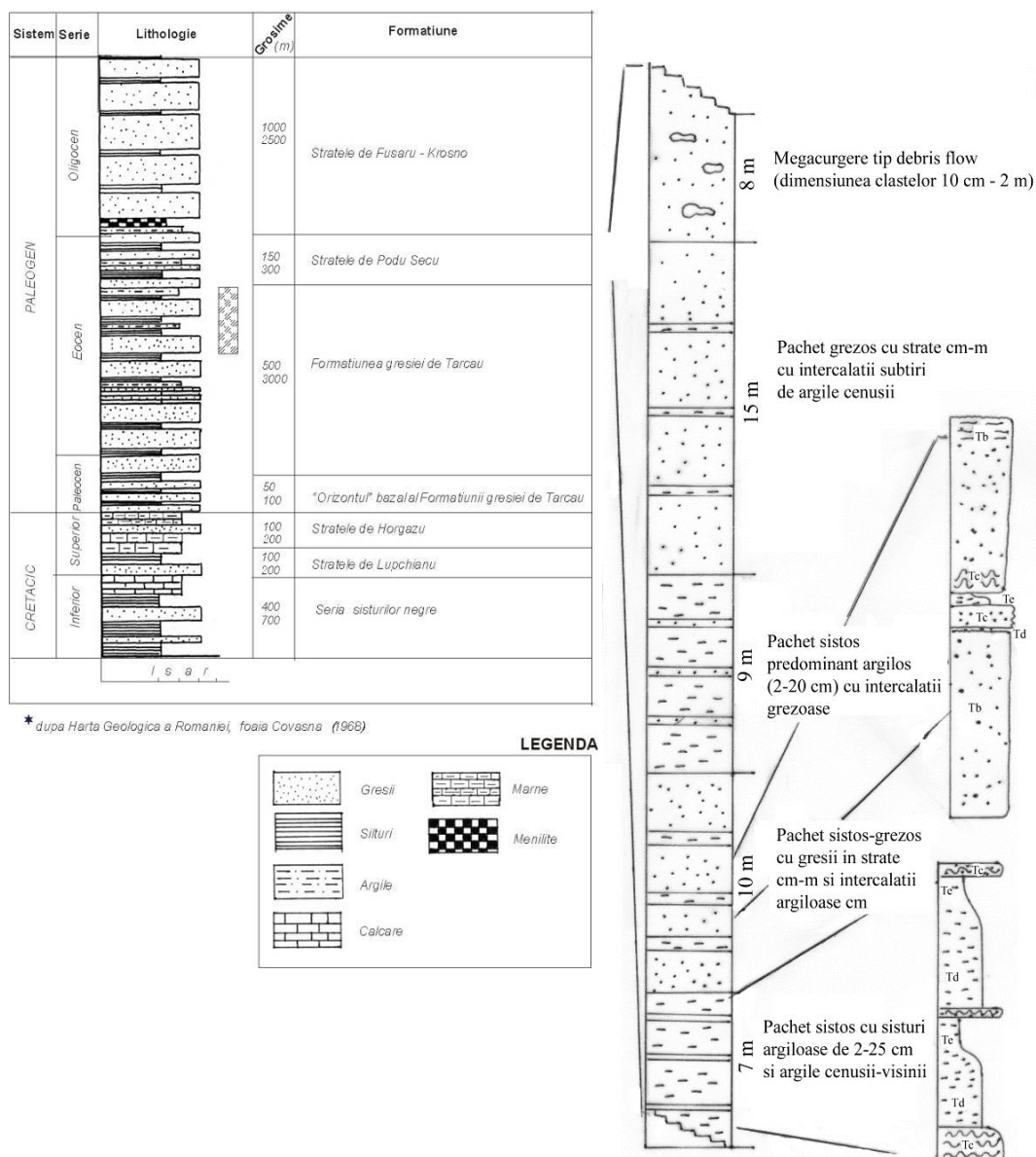
Fig. 2. Stratigraphic setting of the case study (after [6] modified).
