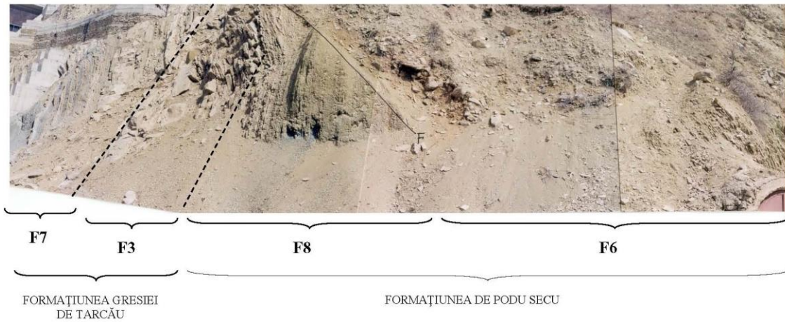
Fig. 4. Panoramic view of the top of Eocene at the contact between Tarcau Sandstone and Podu Secu Formations – left slope of the Buzau Valley, downstream of the Siriu dam, in the road curve adjacent to the base of dam overflow.
