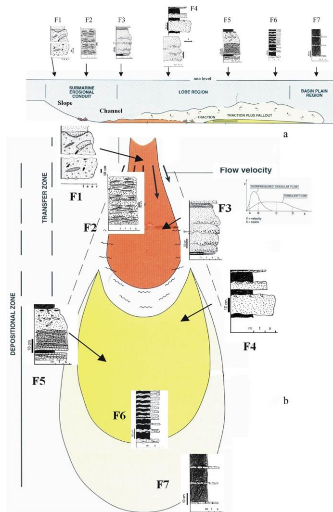
Fig. 12. Distribution of sedimentary facies: a – between slope and basinal plain; b – within depositional transfer zones of turbiditic system according to [12] in [7].
