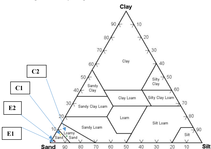
Figure 6. Fitting of the four sand samples within the C-S-A ternary diagram: E2 (black dot), E1 (burgundy dot), C2 (green dot) and C1 (yellow dot)
